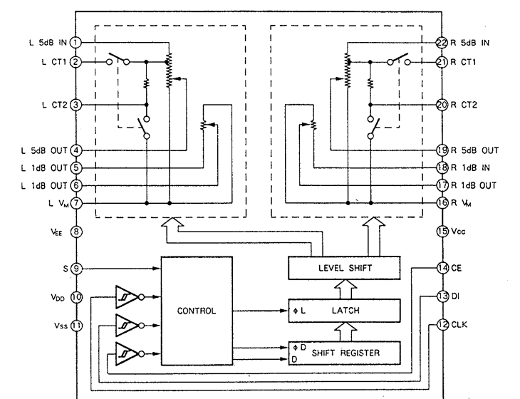
IC304 LC7535
