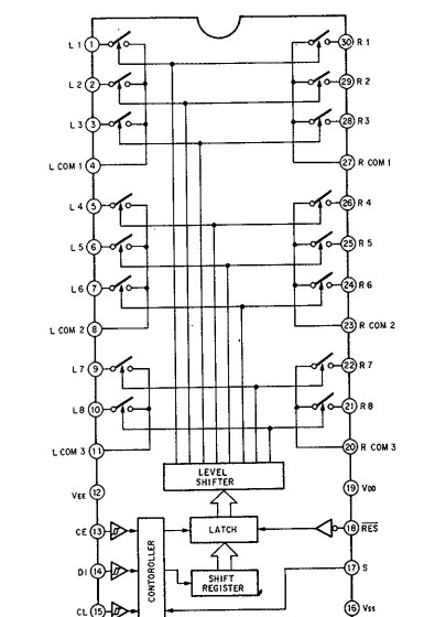
IC402 LC7822
