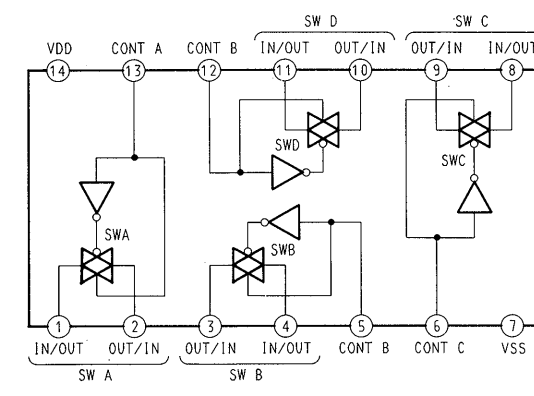
IC301 LC4966
